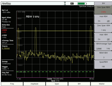
100ms Zero Span Time
