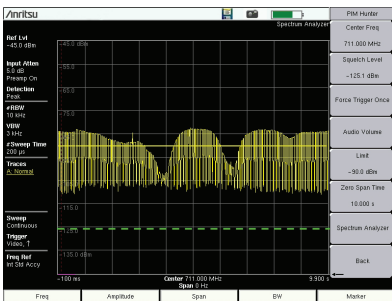
10 sec Zero Span Time
